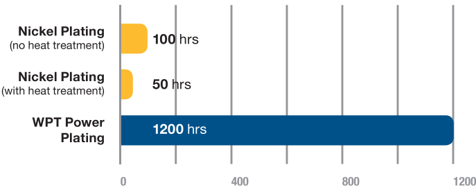
WPT Power FMCP Plating Salt Spray Test
