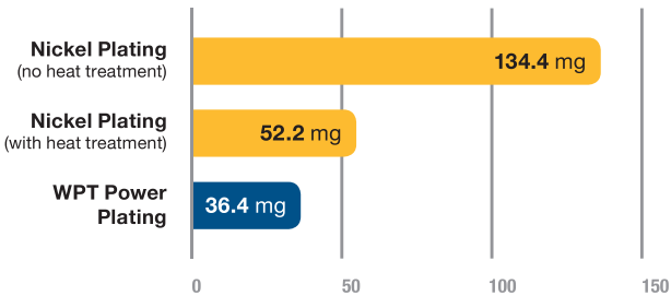
WPT Power FMCP Plating Wear Rates*
